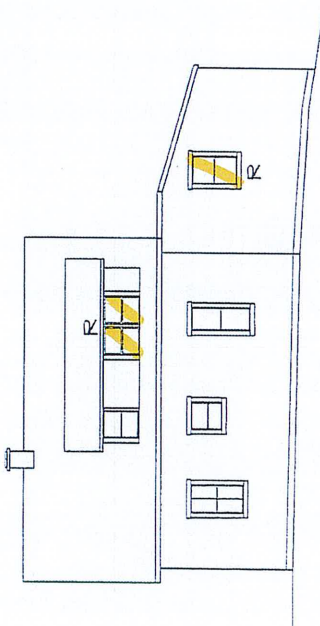
(E) WEST ELEVATION SCALE: 3/16" = 1'-0"
