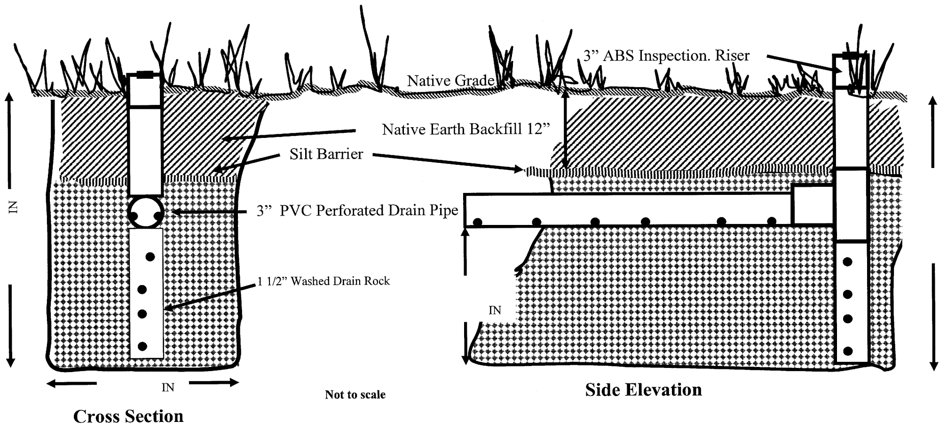
Standard In-Ground Trench
