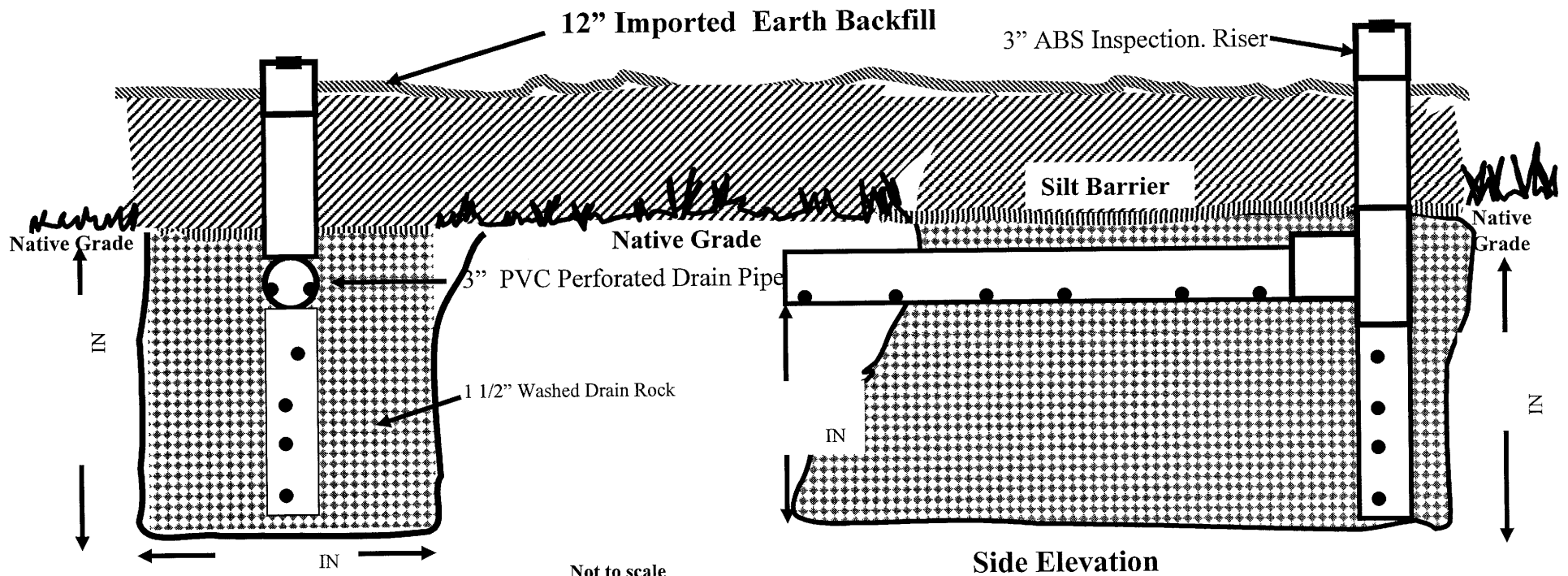
Cross Section
